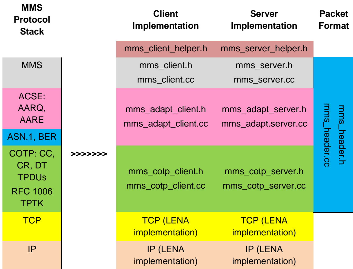
Figure 5.4 - Implementation of the MMS protocol stack for MMS client and MMS server
