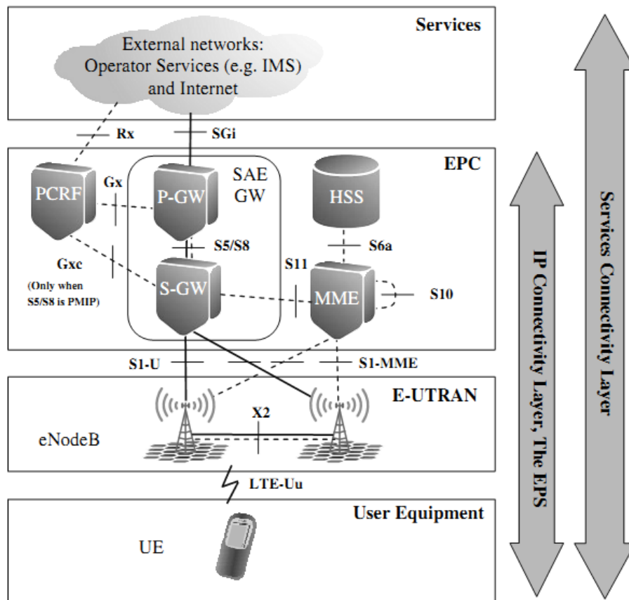
Figure 2.18 – LTE network architecture, copied from [27]
