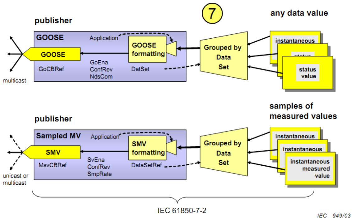
Figure 2.4 – peer-to-peer data value publishing model, copied from [4]
