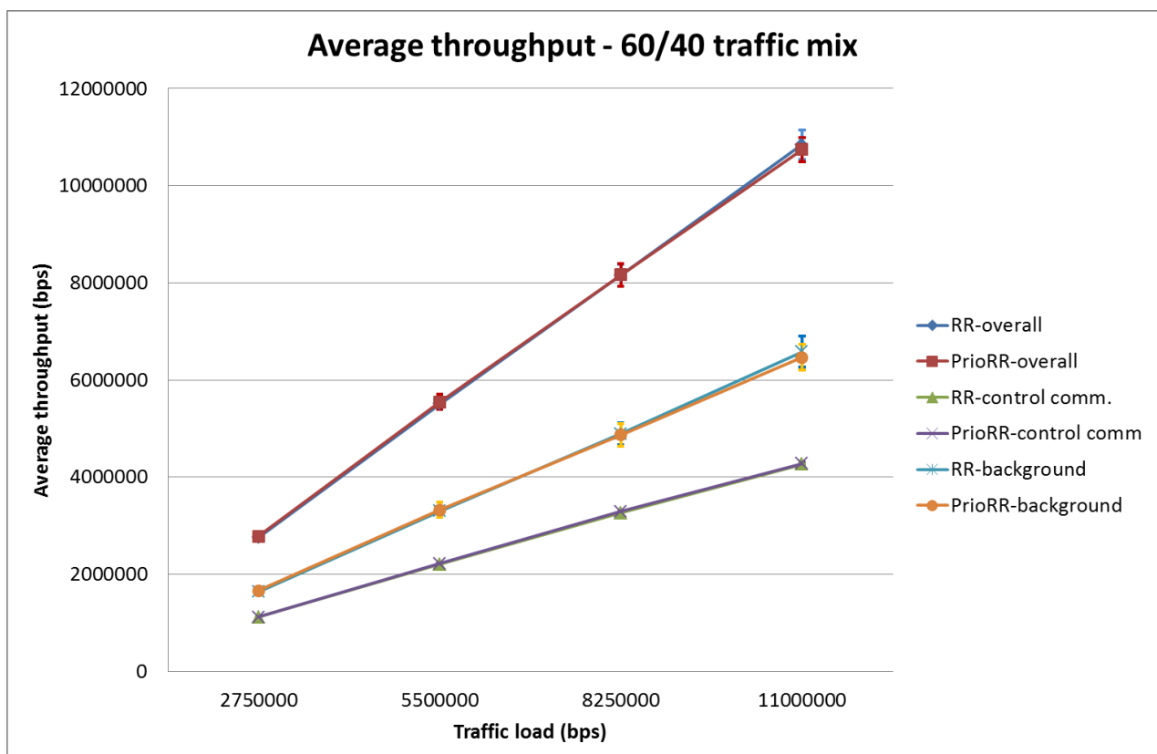
Figure 6.11 – Average throughput performance in 60/40 traffic mix experiment
