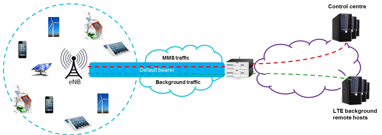
Figure 6.1 – Simulation topology and configuration when using Round Robin scheduler
