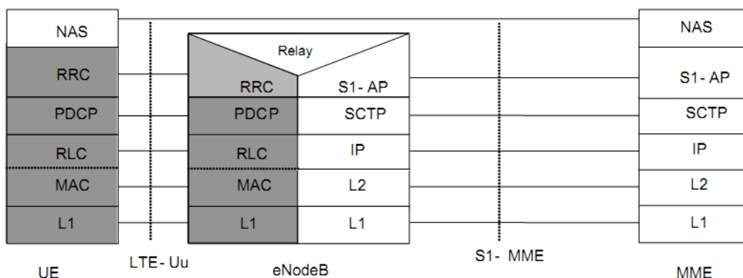
Figure 2.23 – Control plane protocol stack, copied from [28]
