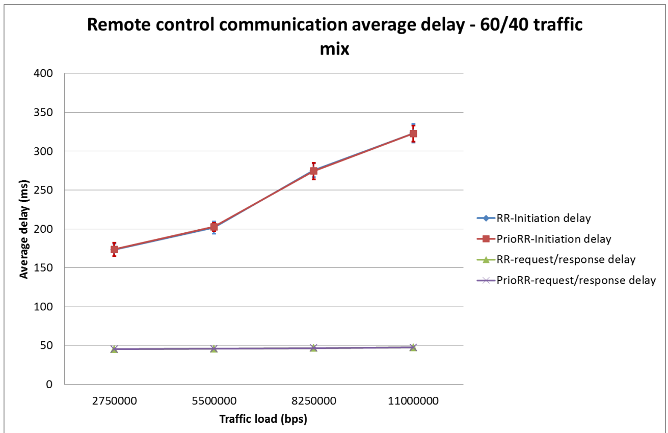
Figure 6.13 – Remote control communication traffic average delay in 60/40 traffic mix experiment
