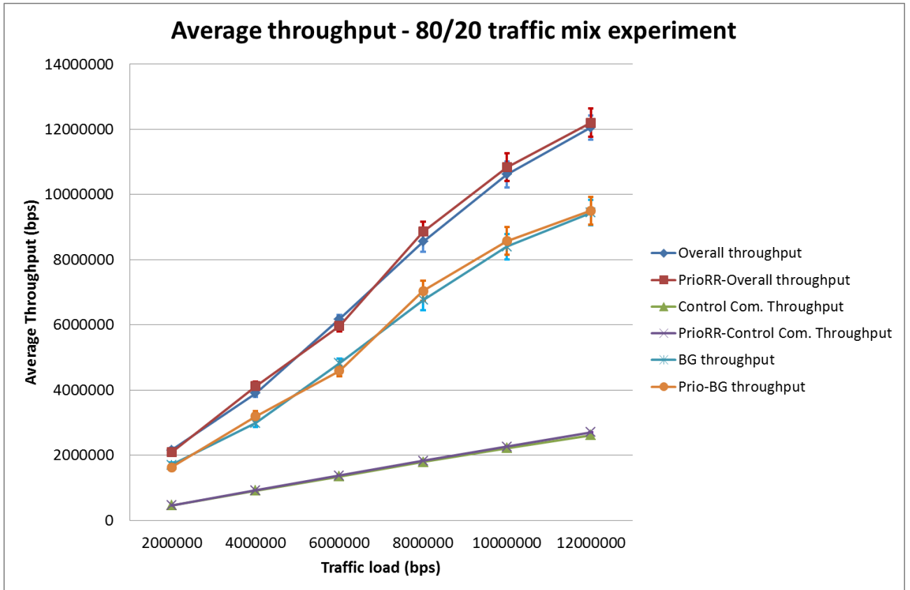
Figure 6.4 – Average throughput performance in 80/20 traffic mix experiment with both Round Robin and Priority-aware Round Robin schedulers
