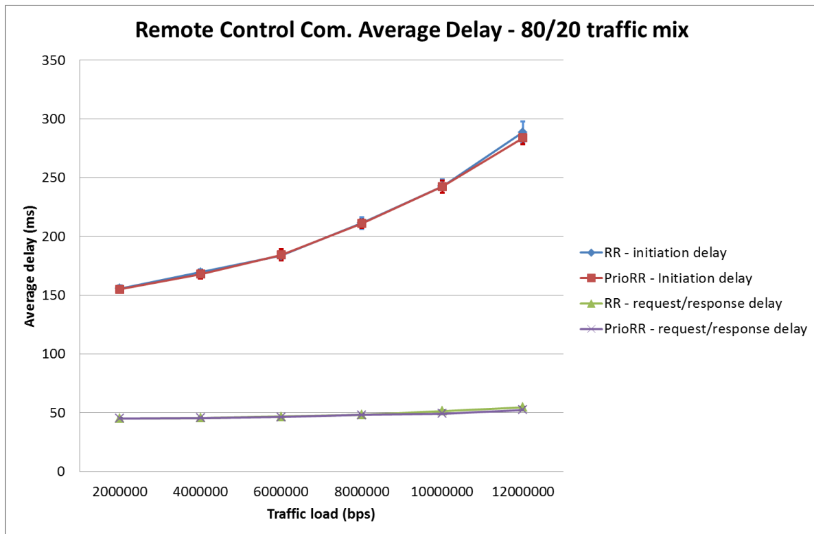
Figure 6.5 – Remote control communication average delay in 80/20 traffic mix experiment
