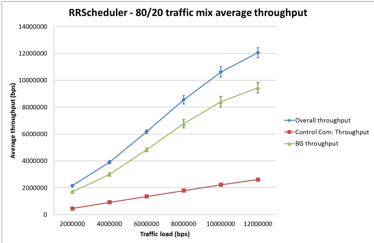
Figure 6.3 – Average throughput performance in 80/20 traffic mix with Round Robin scheduler
