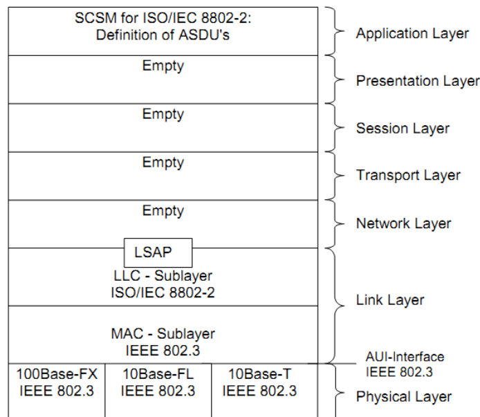
Figure 2.5 – SV mapped to serial unidirectional multi-drop point to point link, copied from [36]
