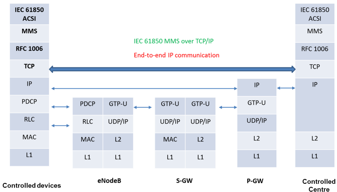
Figure 4.11 – Remote control communication system in distribution grid with the integration of 61850 MMS and LTE
