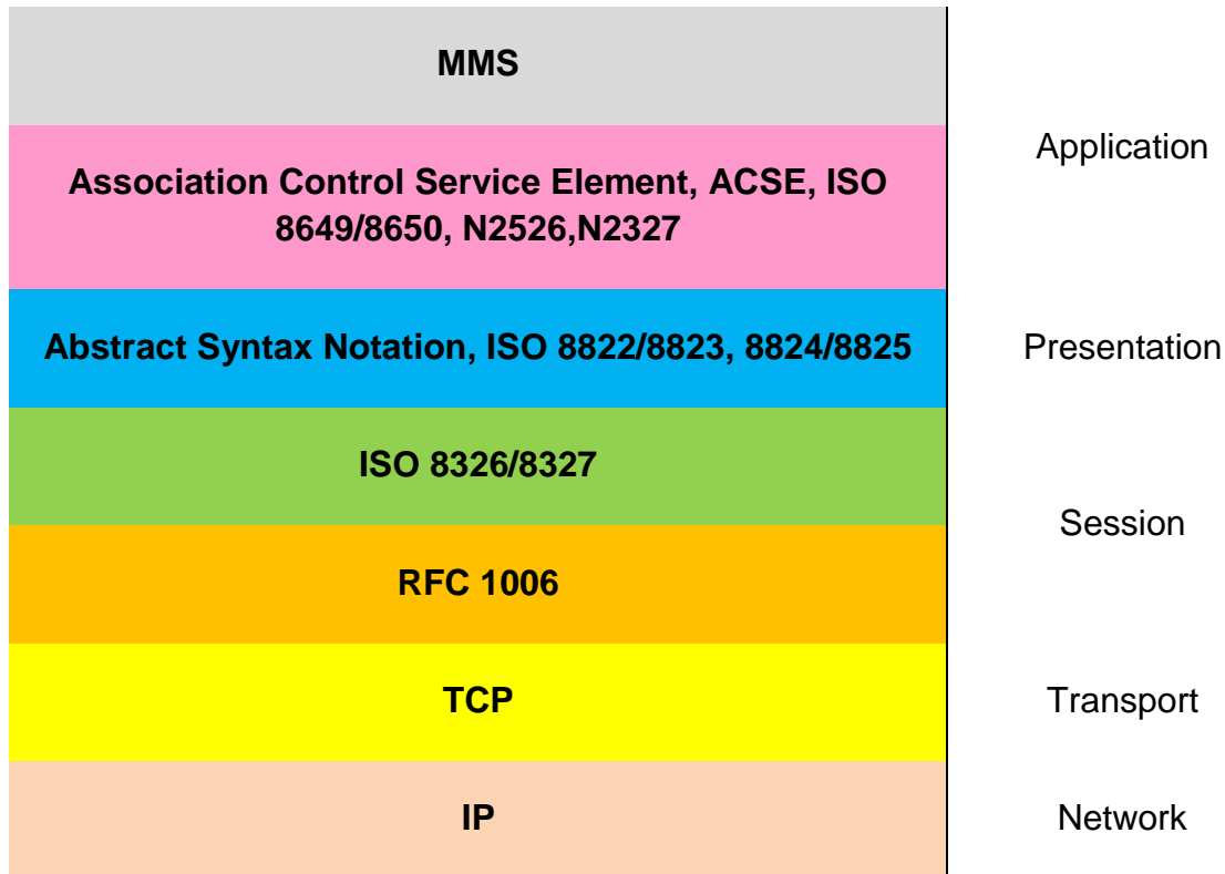
Figure 4.3 - Layer 3-7 of the current MMS communication stack, based on [57][58]
