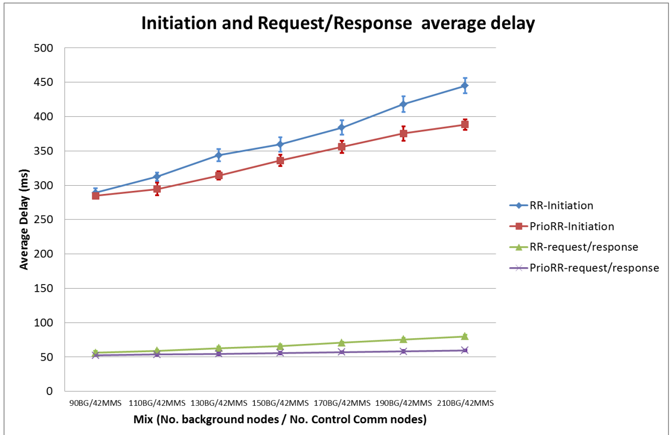
Figure 6.9 – Initiation and Request/Response average delay in traffic overload experiment
