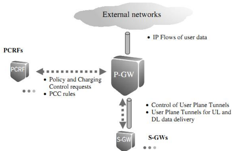
Figure 2.21 – P-GW connections to other logical nodes and main functions, copied from [27]
