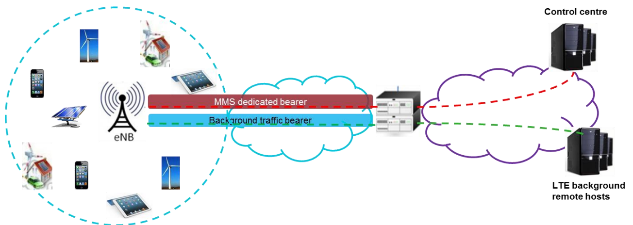
Figure 6.2 – Simulation topology and configuration when using Priority-aware Round Robin scheduler
