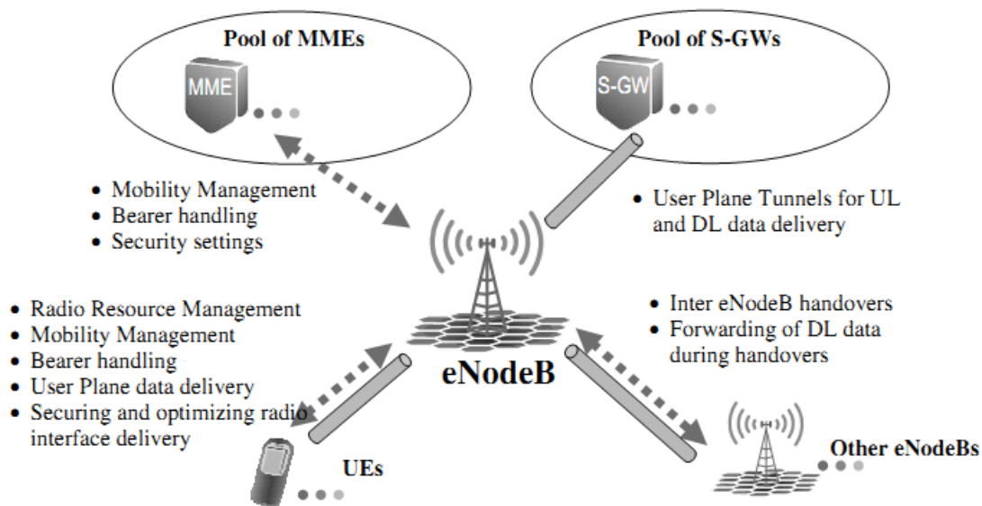
Figure 2. 19 – eNodeB connections to other logical nodes and main functions, copied from [27]
