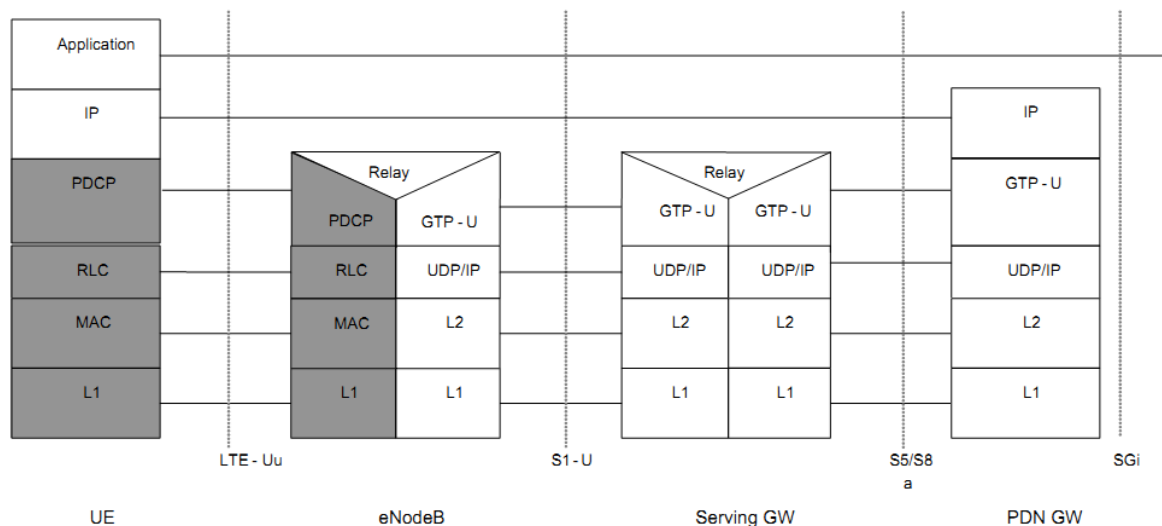
Figure 2.24 – User plane protocol stack, copied from [28]
