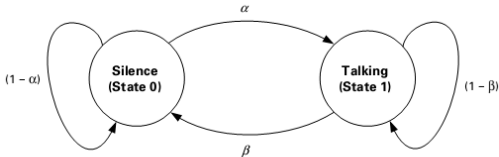
Figure 5.6 – Two-state voice activity model, copied from [60]
