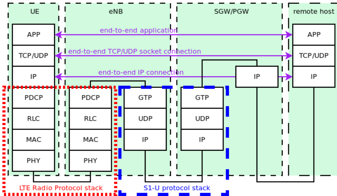
Figure 5.2 - LTE-EPC data plane protocol stack, copied from [56]
