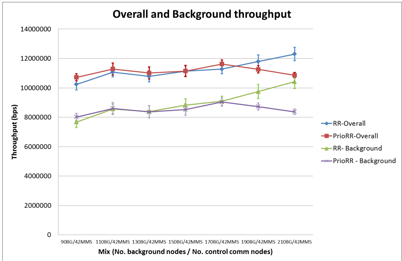
Figure 6.8 – Overall and background throughput in traffic overload experiment
