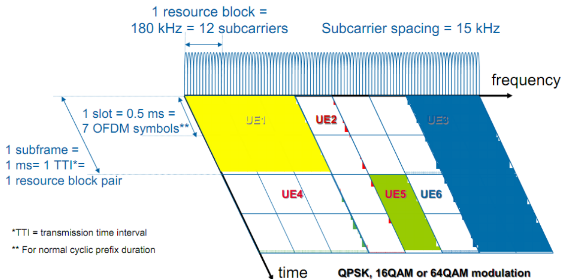
Figure 4.8 - Resource allocation for users using OFDMA, copied from [62]
