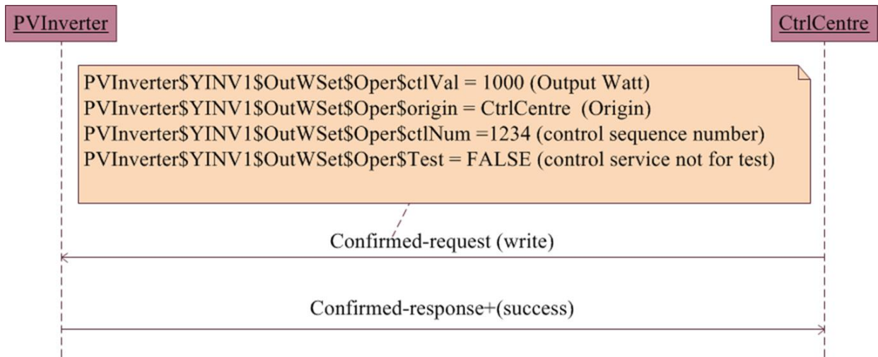
Figure 4.2 – Control centre uses IEC 61850 MMS services to control a PV panel
