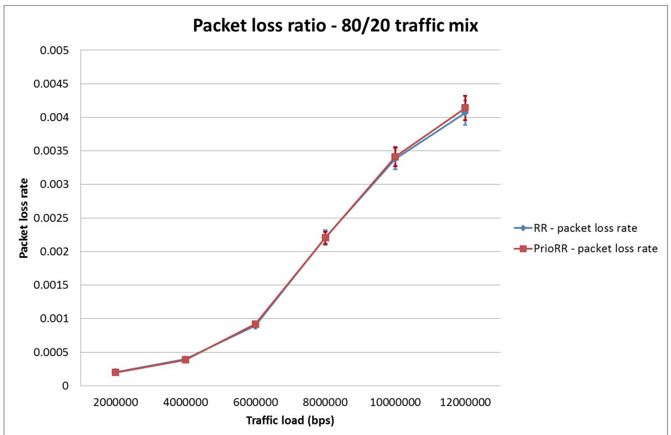
Figure 6.6 – Packet loss ratio in 80/20 traffic mix experiment
