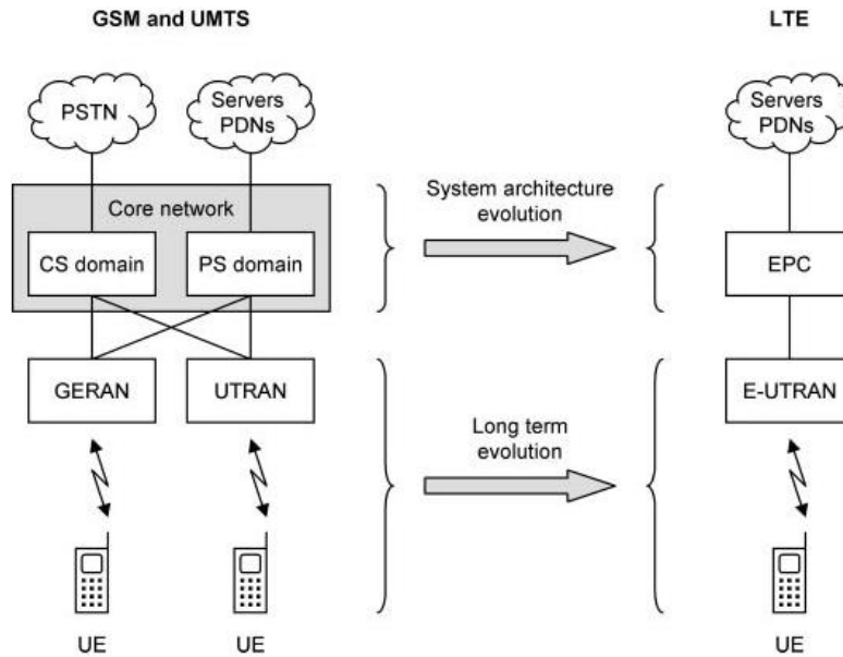
Figure 2.17 – Evolution of the system architecture from GSM and UMTS to LTE, copied from [24]
