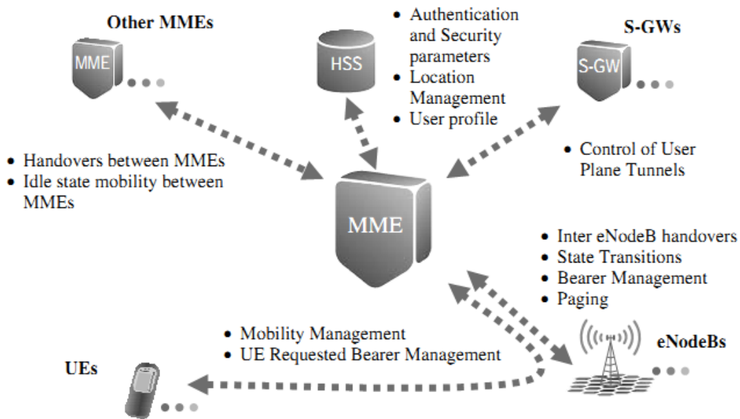
Figure 2.20 – MME connections to other logical nodes and main functions, copied from [27]
