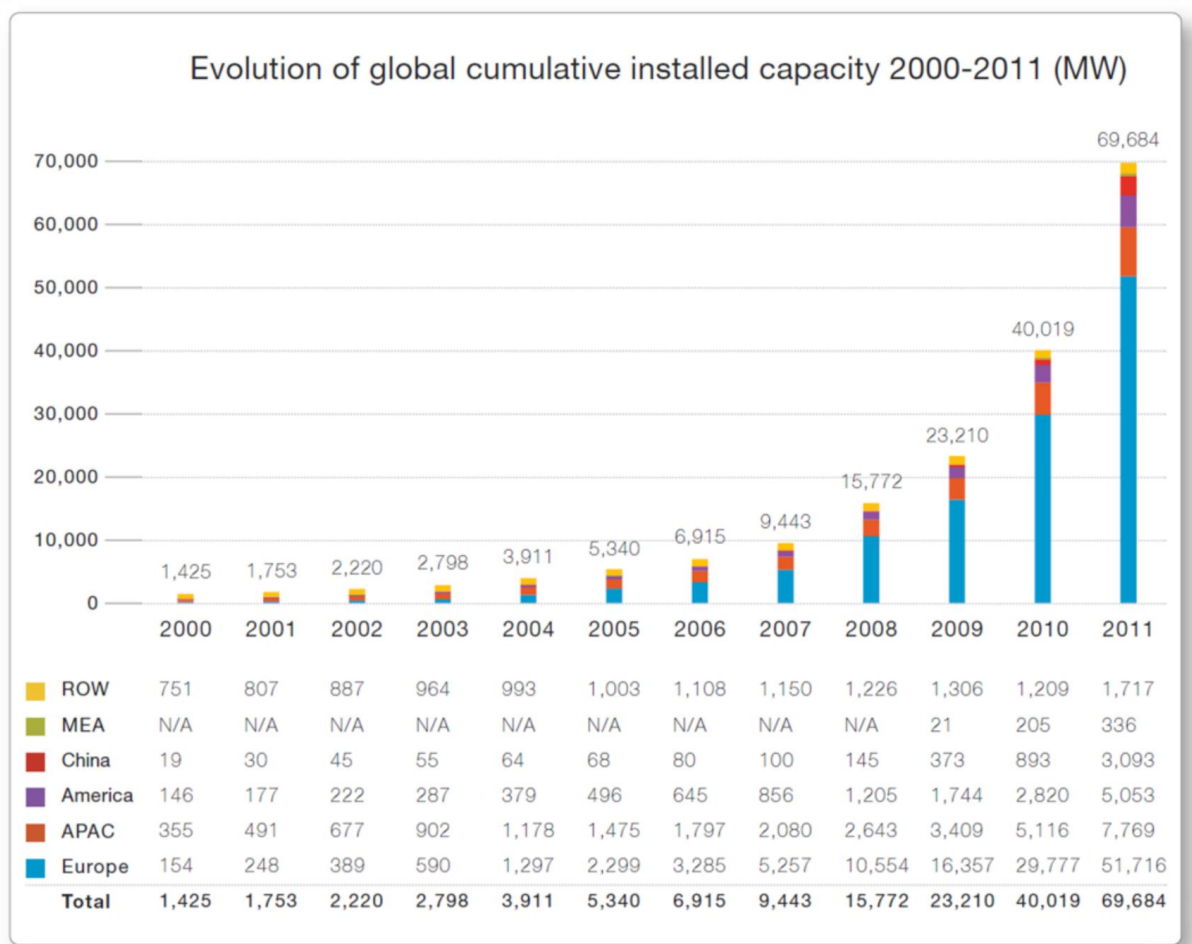
Figure 2.13 – Evolution of the cumulative installed PV capacity, copied from [55]
