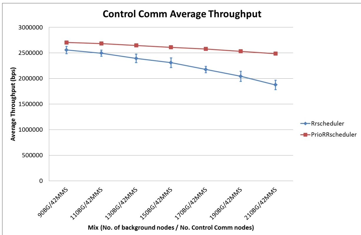
Figure 6.7 - Control communication throughput in traffic overload experiment
