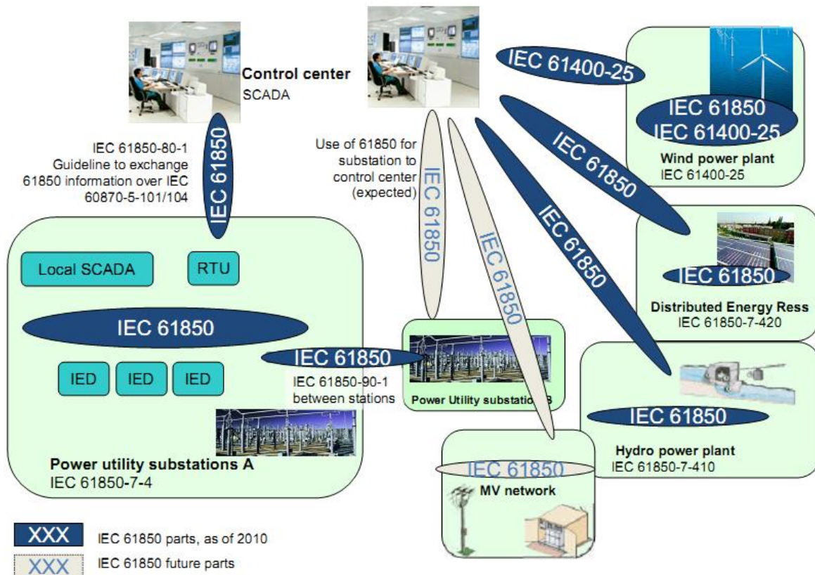
Figure 2.1 – Scope of application of IEC 61850, copied from [11]
