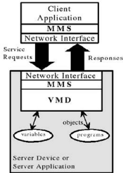
Figure 2.6 – VMD communication model between MMS client and server, copied from [54]
