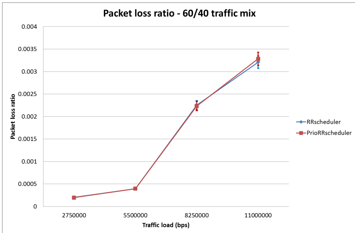
Figure 6.12 – Packet loss ratio in 60/40 traffic mix experiment
