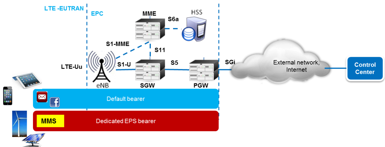
Figure 4.10 – LTE dedicated bearer for remote control communication
