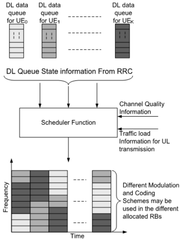
Figure 4.9 – Generic view of LTE MAC scheduler, copied from [27]
