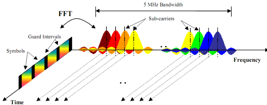
Figure 4.7 - Sub-carrier overlap in OFDMA, copied from [62]
