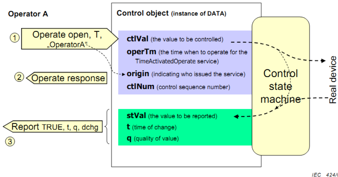
Figure 2.14 – Principle of the control model, copied from [19]
