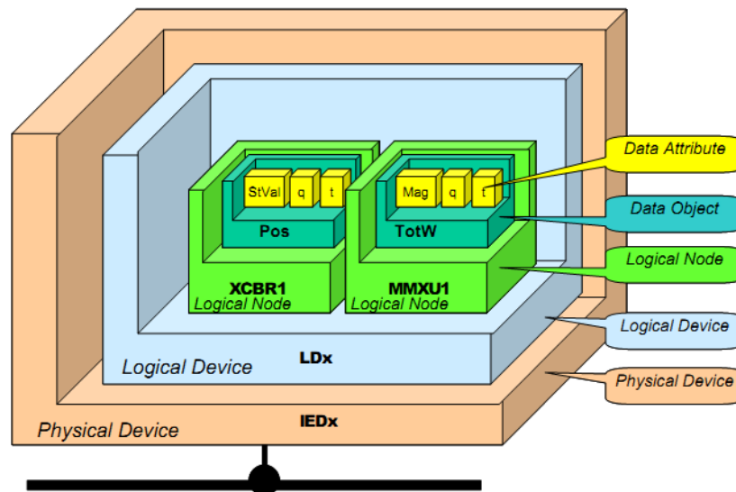
Figure 2.2 – Links between IEC 61850 parts, copied from [11]
